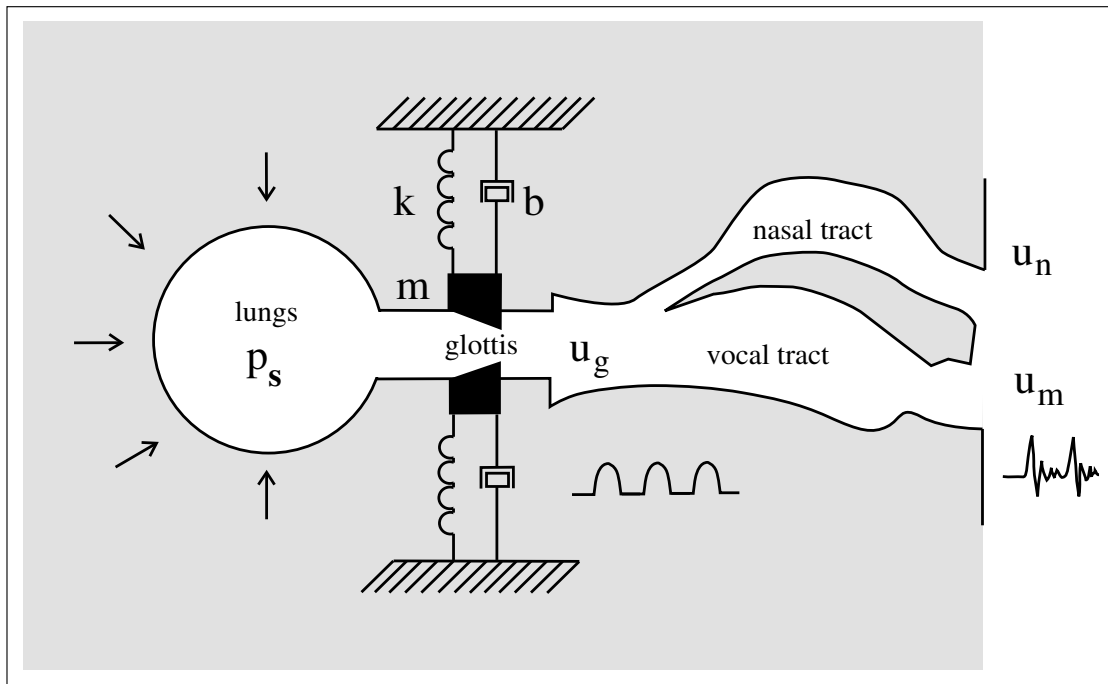
Figure 1.1: Schematic diagram of speech production.
